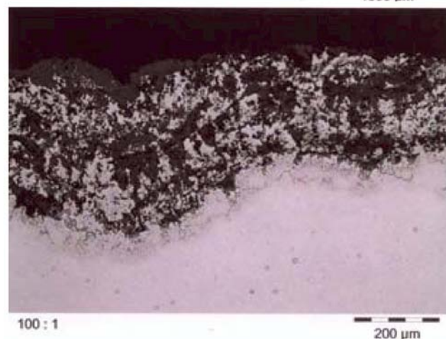
Figure 09: Micro cuts of Nimonic with high-temperature corrosion.
