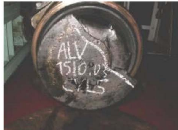
Figure 12: Catastrophic failure of a repaired valve spindle (RTA 72 Nimonic-type 740 hrs after repair)
