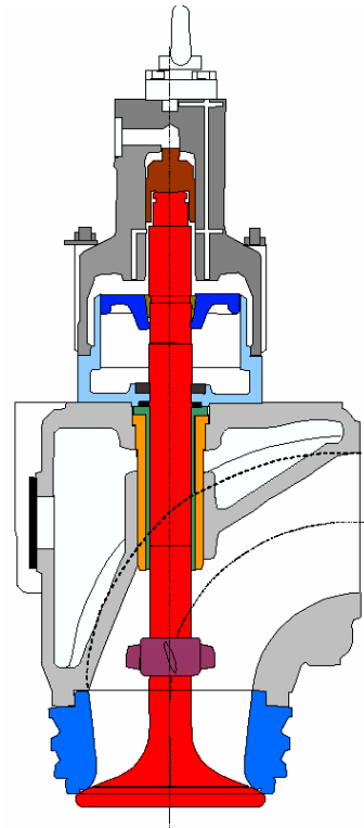
Figure 01: Main components of an exhaust valve
