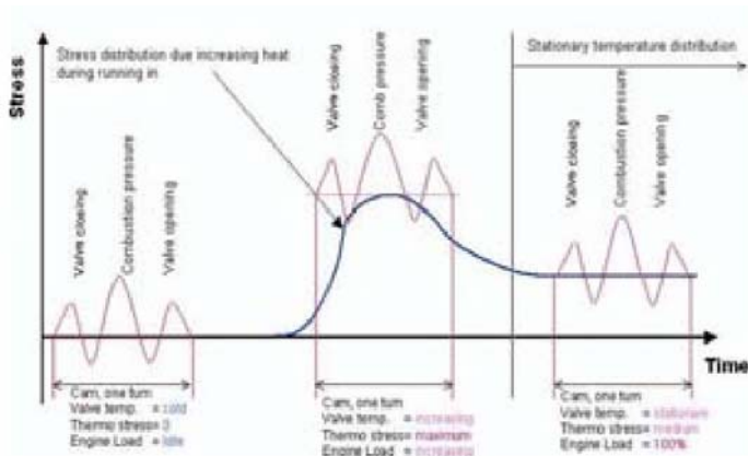
Figure 11: Mechanical and thermal load as function of running in and stationary operation
