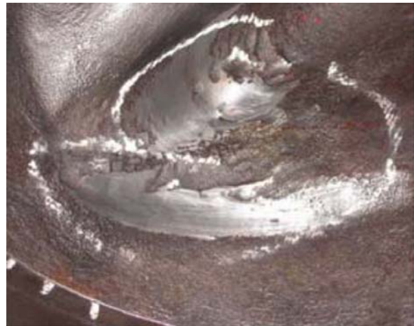
Figure 05: Low temperature corrosion of valve housing (MC-type 43,700 hrs)
